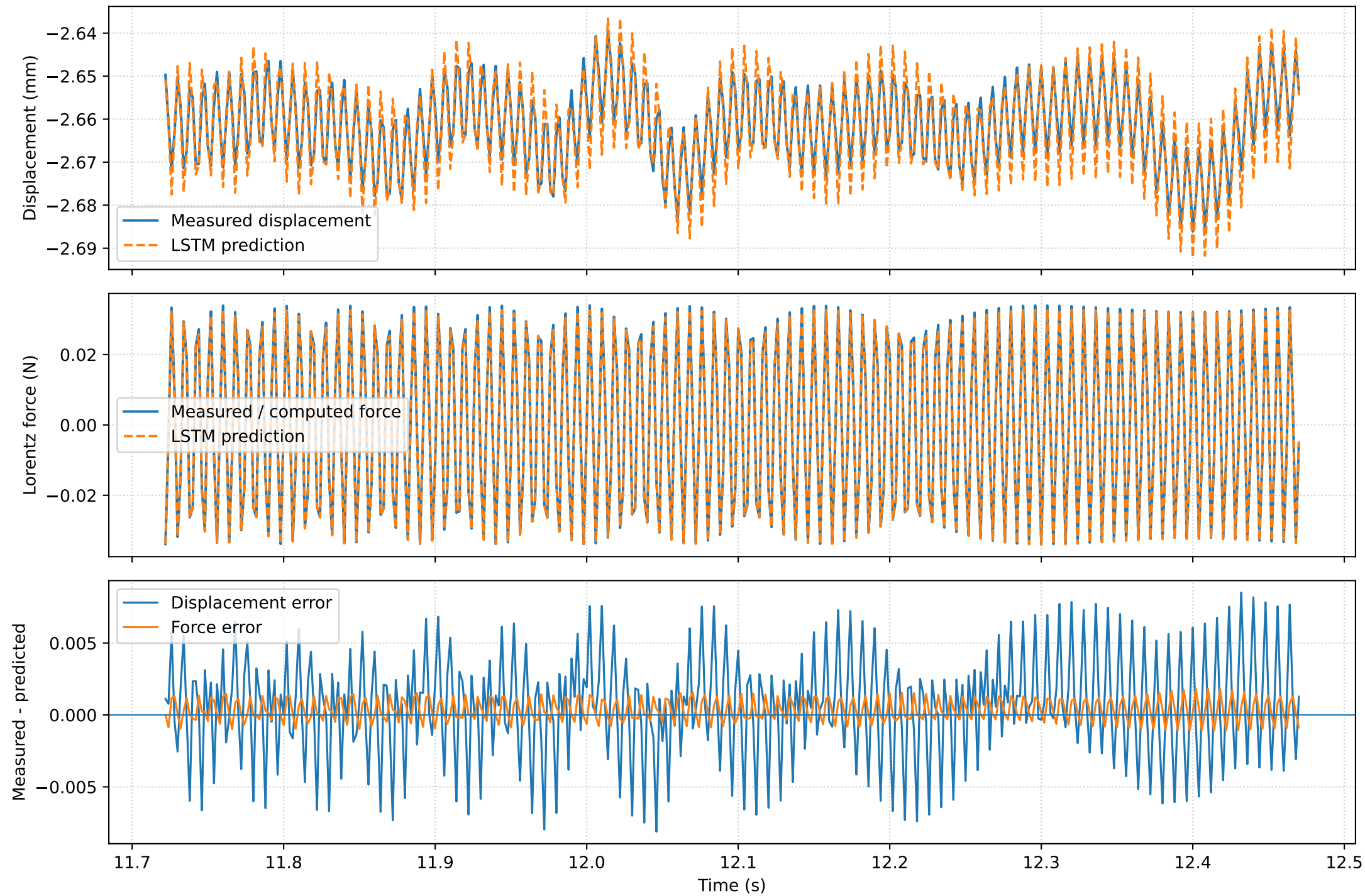
Zoomed LSTM tracking: Chirp_1 | center = 12.096 s | window = 0.750 s
